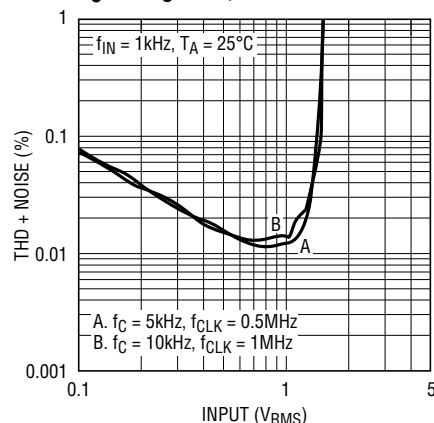
THD + Noise vs Input Voltage; V_S = \text{Single } 5V, AGND = 2V
