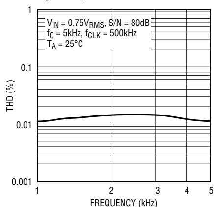
THD vs Frequency; V_S = \text{Single } 5V, AGND = 2V
