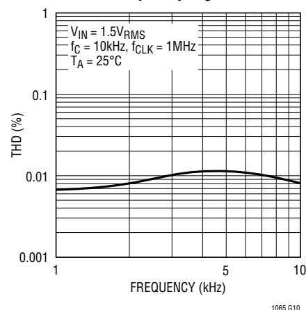
THD vs Frequency; V_S = \pm 5V
