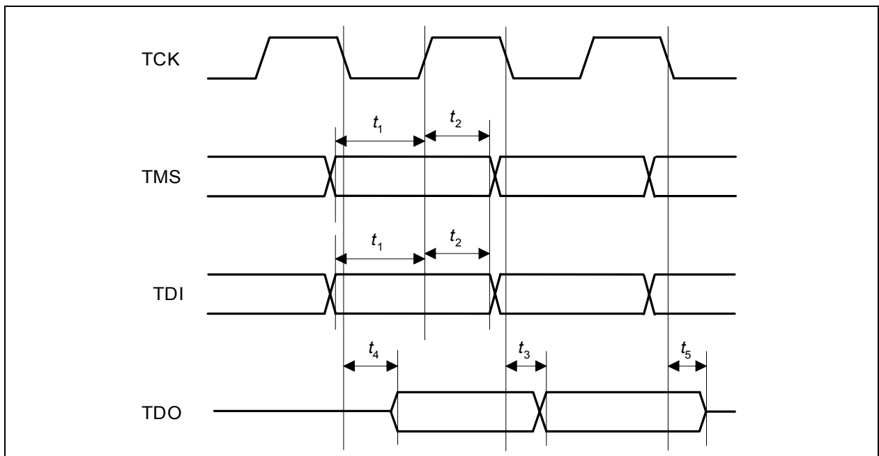
Figure 44 JTAG Timing
