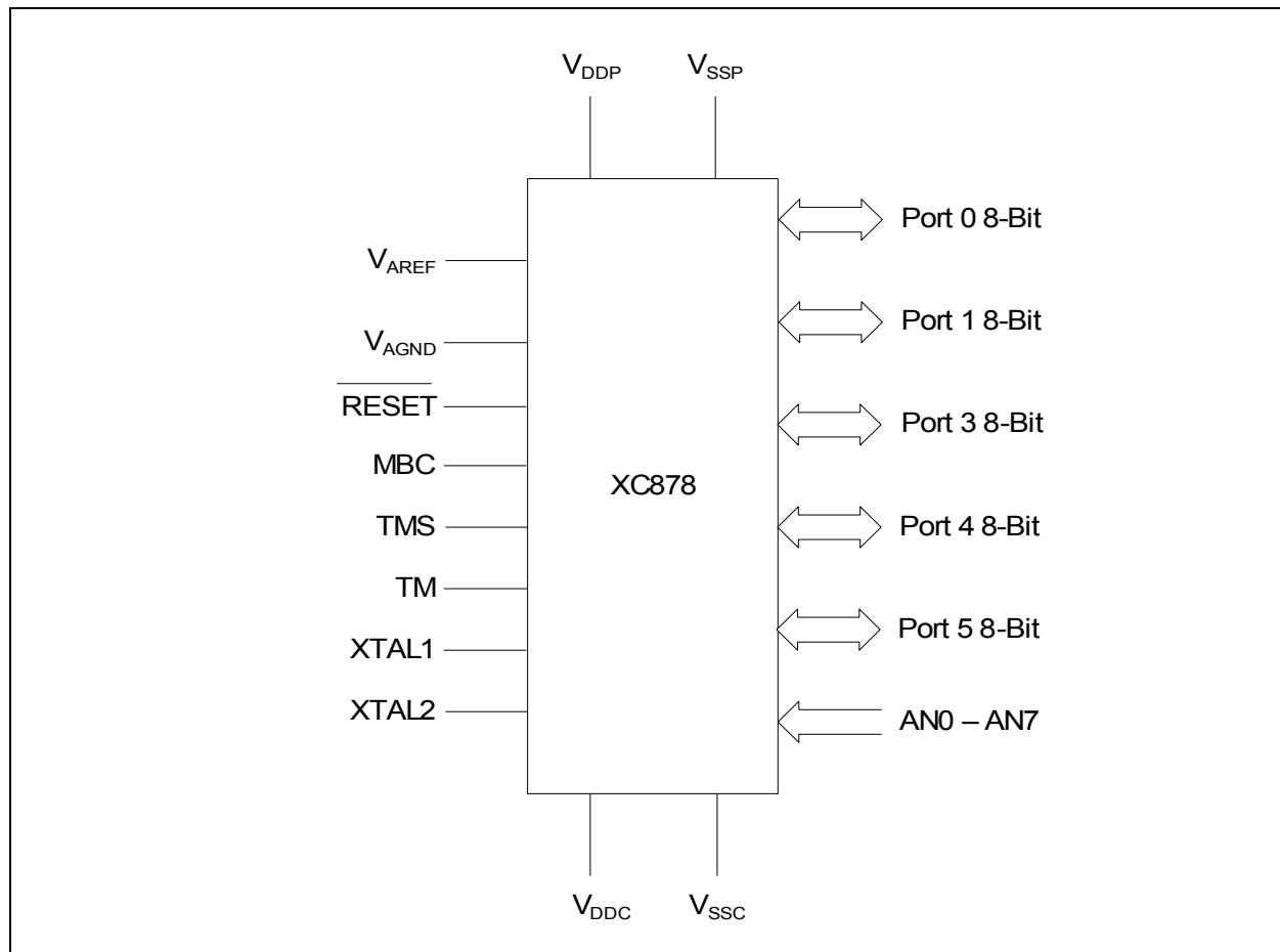
Figure 3 XC878 Logic Symbol
