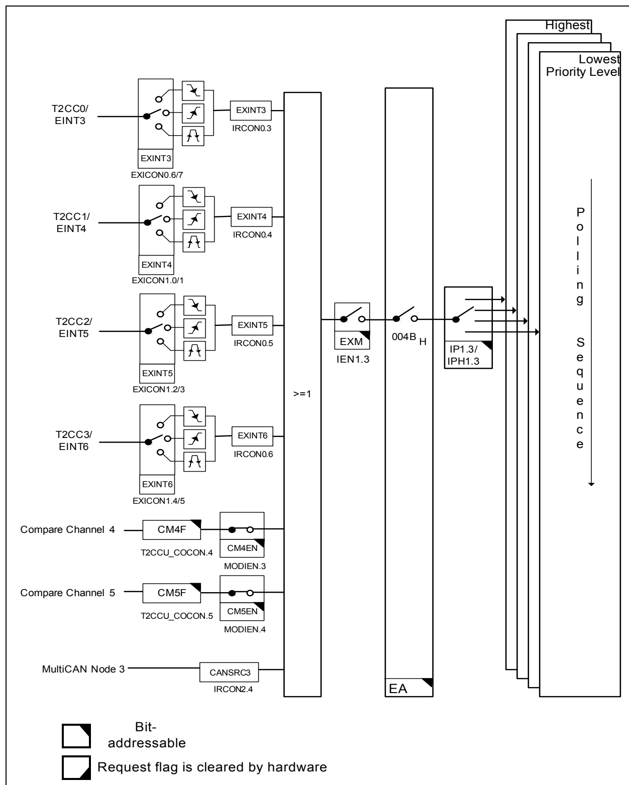
Figure 15 Interrupt Request Sources (Part 4)
