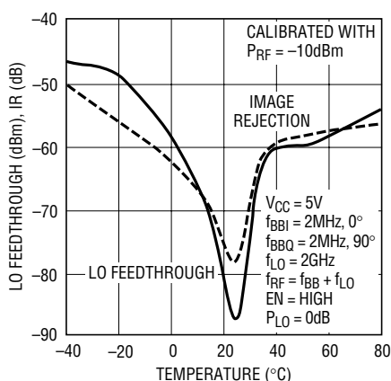
Figure 15. LO Feedthrough and Image Rejection vs Temperature After Calibration at 25°C
