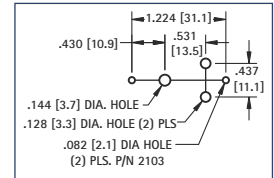
Mounting Detail
