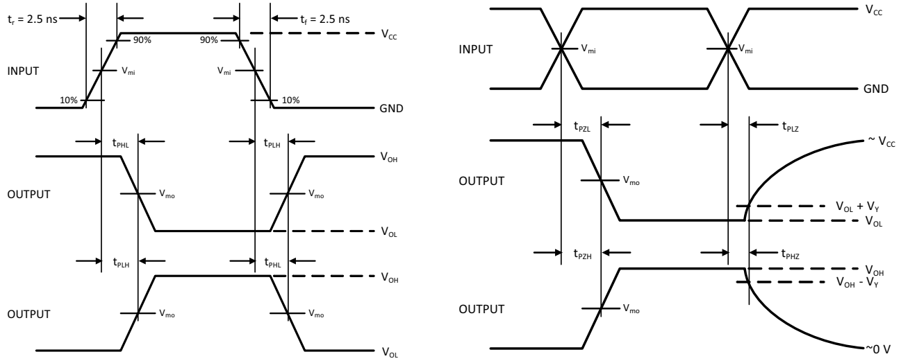
Figure 2. Switching Waveforms
