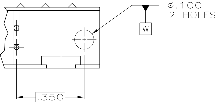
VIEW W-W
