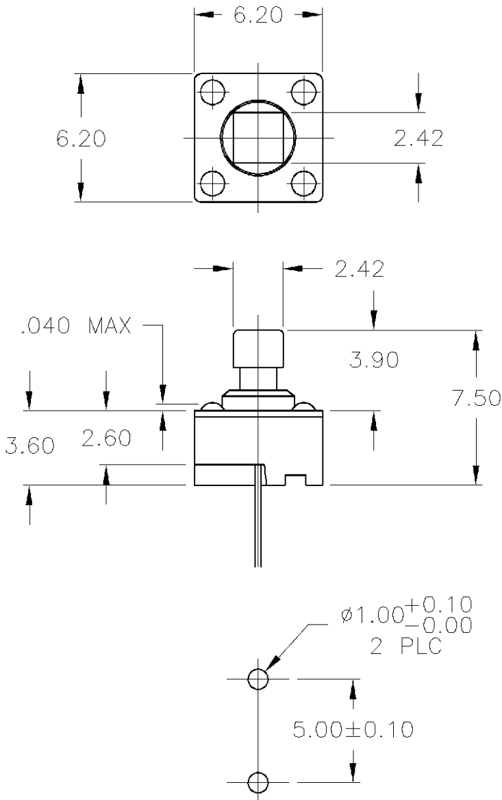
PCB MOUNTING HOLE DIMENSIONS
