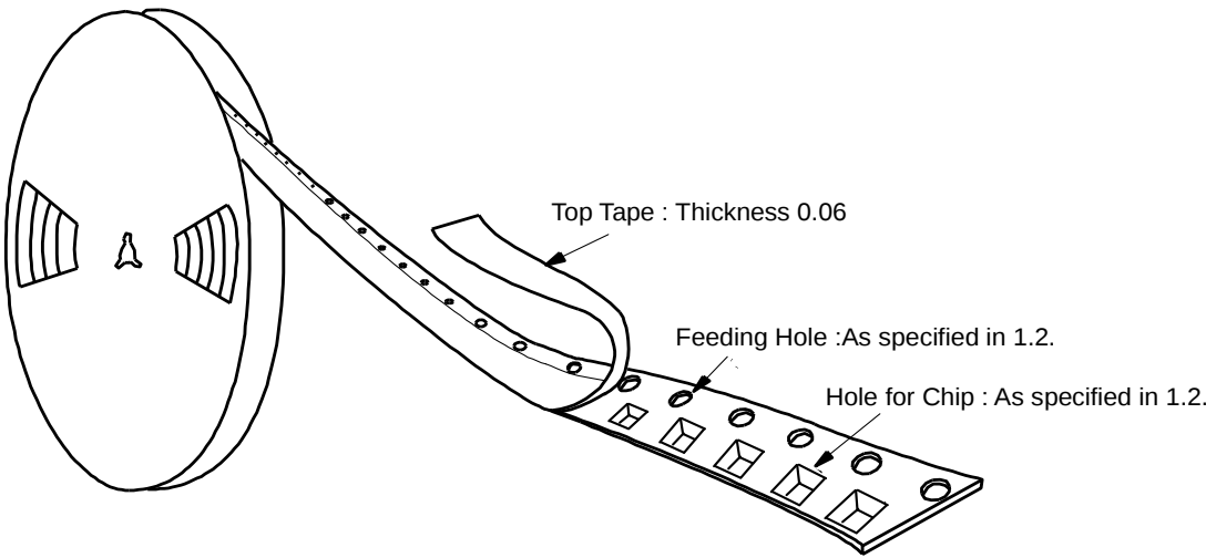
Fig.3 Taping Diagram
