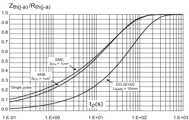
Figure 3. Relative variation of thermal impedance junction to ambient versus pulse duration (epoxy printed circuit FR4, L_{leads} = 10 mm, S_{Cu} = 1\text{cm}^2 )
