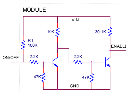
Figure 48. Remote On/Off Implementation.
