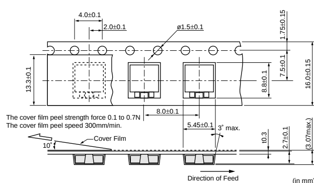
CSBFB_J 700-1250kHz
