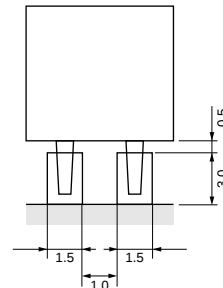
CSBFB_J (700-1250kHz)
