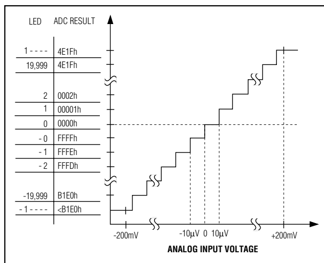
Figure 18. MAX1499 Transfer Function, \pm 200\text{mV} Range
