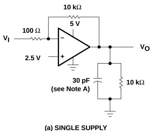
(a) SINGLE SUPPLY
