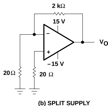
Figure 2. Noise-Voltage Test Circuit
