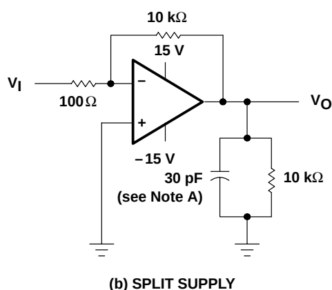
(b) SPLIT SUPPLY
