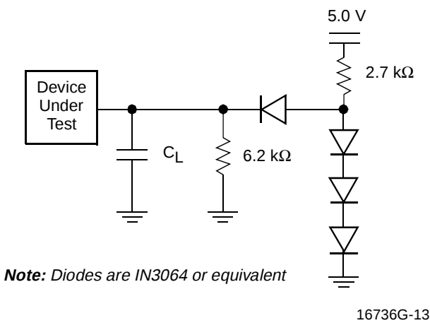
Figure 7. Test Setup
