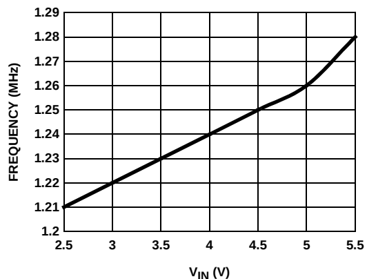
FIGURE 20. FREQUENCY (1.2MHz) vs V_{IN}
