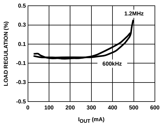
FIGURE 18. LOAD REGULATION - 3.3V TO 8V
