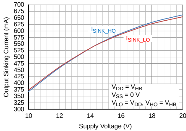
Figure 23. Output Sinking Current vs. Supply Voltage ( V_{DD} )
