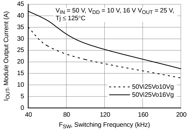
Figure 33. Static SOA, V_{IN} = 50\text{ V}
