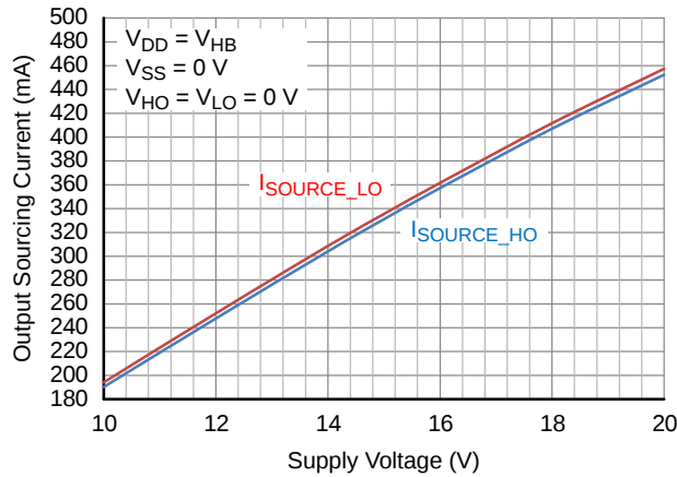
Figure 21. Output Sourcing Current vs. Supply Voltage ( V_{DD} )
