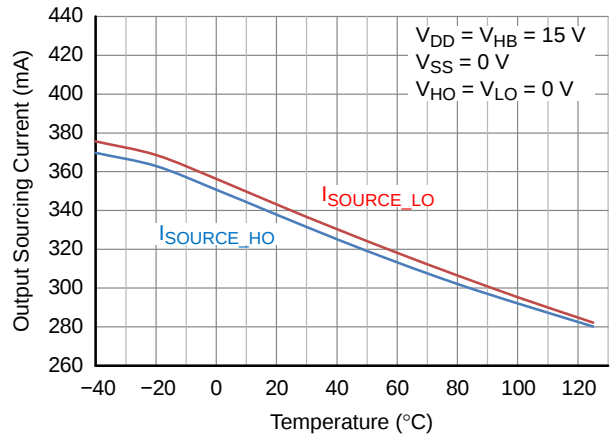
Figure 22. Output Sourcing Current vs. Temperature
