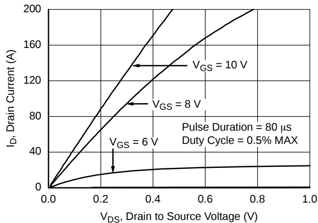
Figure 50. On-Region Characteristics
