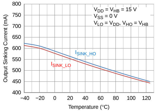
Figure 24. Output Sinking Current vs. Temperature
