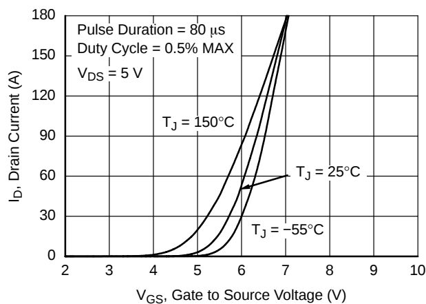
Figure 42. Transfer Characteristics
