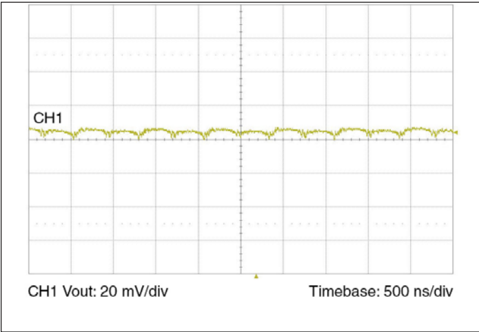
Figure 6 — Output voltage ripple at full load and 48 V F with 47 μF ceramic POL bypass capacitance and 20 nH distribution inductance.
