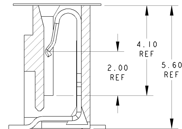
SECTION A - A (FOR EVEN POSITION CONTACTS) SCALE 10:1
