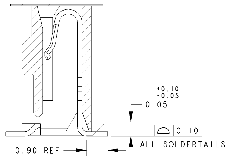
SECTION B - B (FOR ODD POSITION CONTACTS) SCALE 10:1
