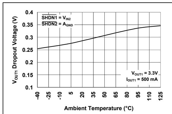
FIGURE 2-19: V_{OUT1} Dropout Voltage vs. Ambient Temperature.
