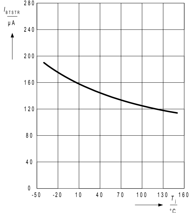
Start-up bootstrap charging current vs. junction temperature
