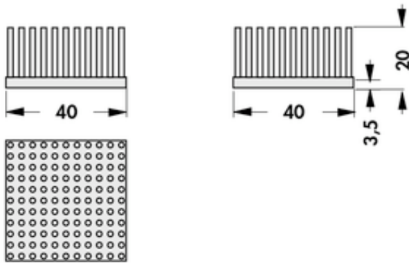
40 x 40 x 20 mm, pin heatsinks quadratic
