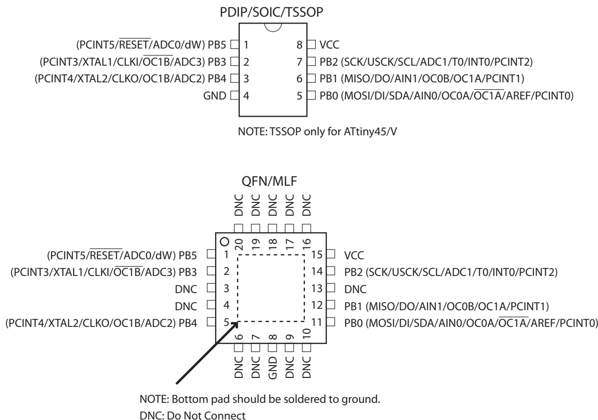
Figure 1-1. Pinout ATtiny25/45/85
