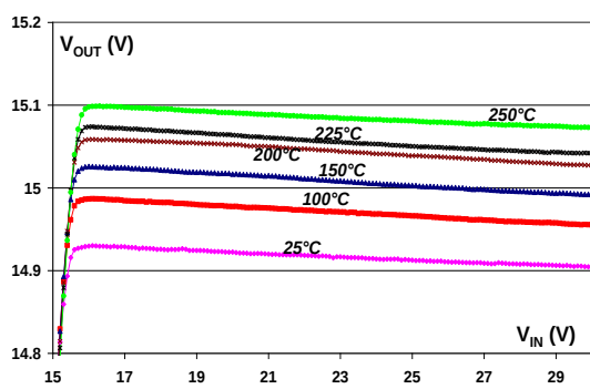
Figure 5: V_{out} vs. V_{in} over T^\circ
