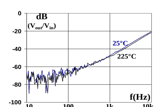
Figure 6: Input ripple rejection ( C_{out} = 1\mu F )
