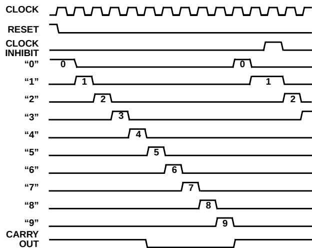
FIGURE 3. CD4017BMS
