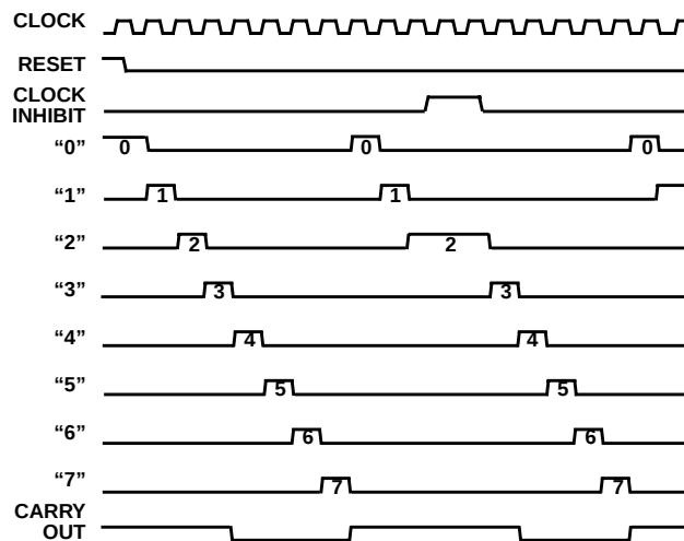
FIGURE 4. CD4022BMS
