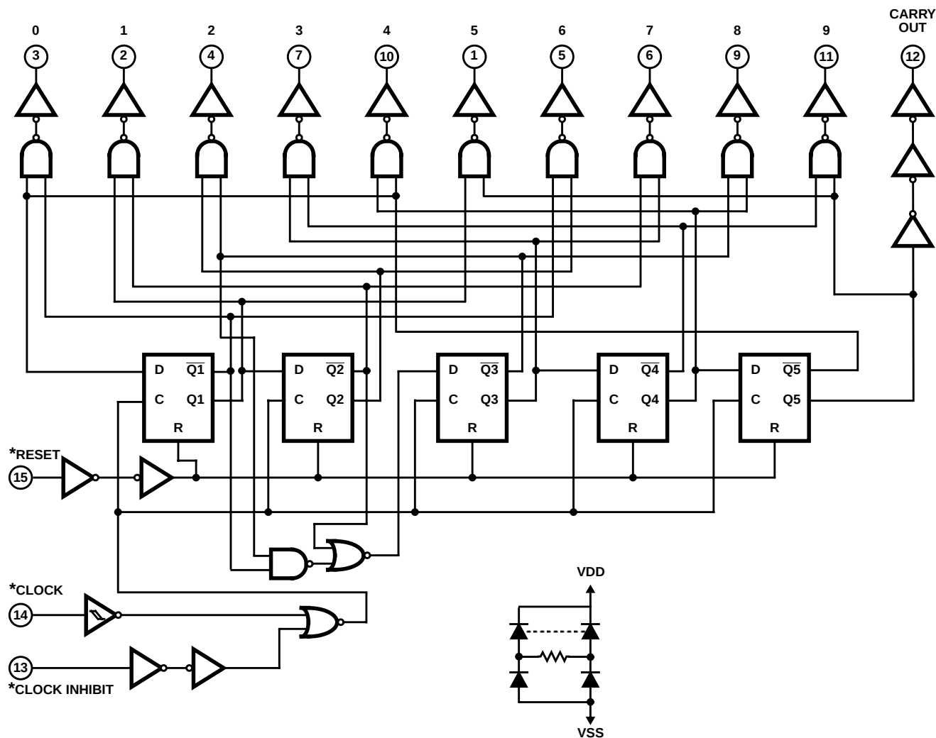
FIGURE 1. CD4017BMS
