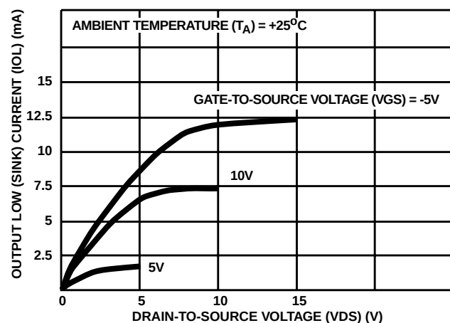
FIGURE 6. MINIMUM OUTPUT LOW (SINK) CURRENT CHARACTERISTICS
