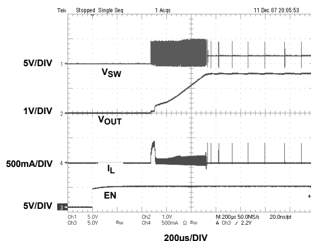
FIGURE 7. SOFT-START ( V_{IN} = 4.2V , V_{OUT} = 1.6V , I_{OUT} = 1mA )
