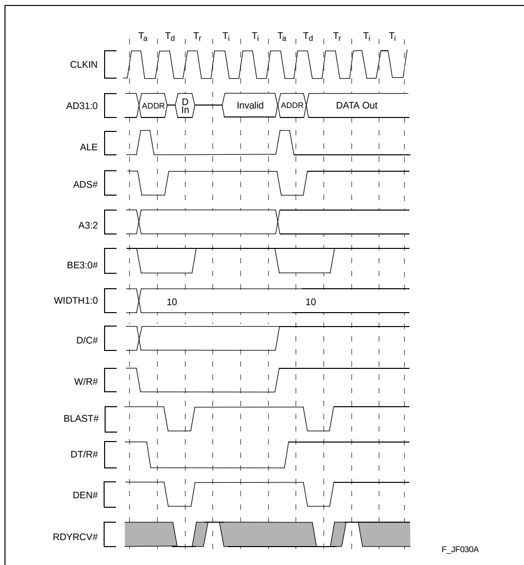
Figure 42. Non-Burst Read and Write Transactions Without Wait States, 32-Bit Bus
