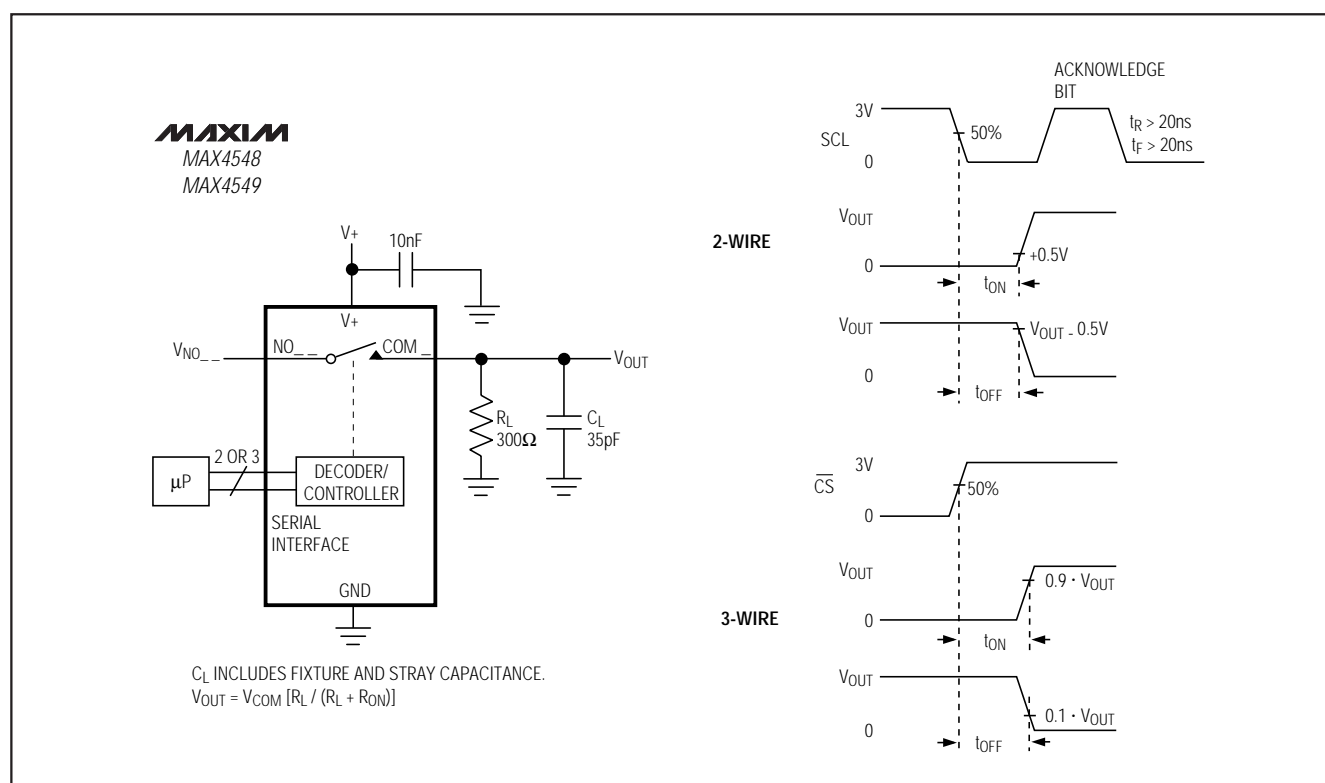
Figure 1. Switching Times
