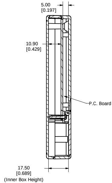
SECTION A-A (Side Inside Assembly)
