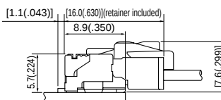
PA Receptacle + PA side entry type header (SMT) (Retainer mountable type)
