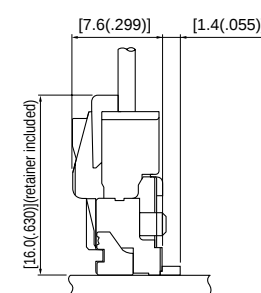
PA Receptacle + PA Header (Retainer mountable type)
