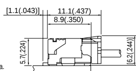
PA Receptacle + PA side entry type header (SMT) (Standard type)
