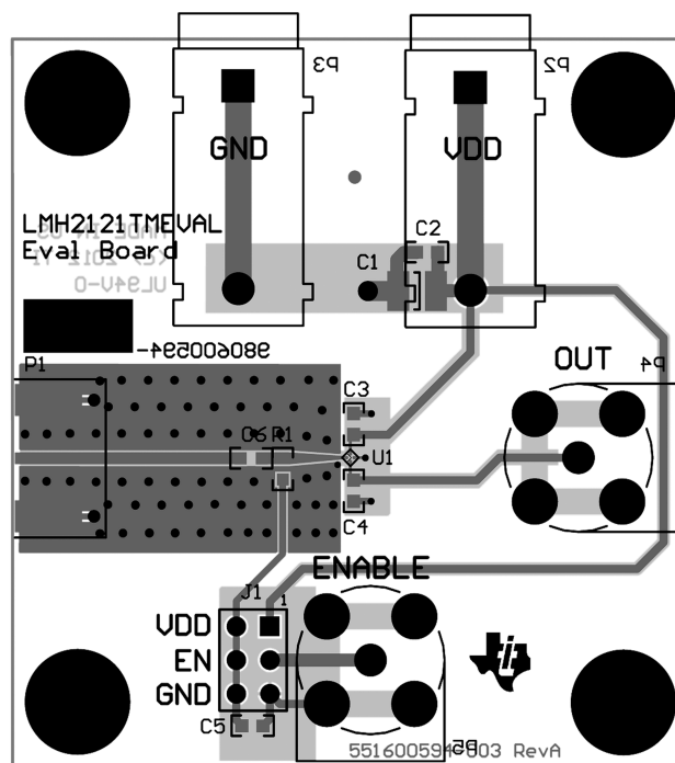
Figure 9. Board Layout of Evaluation Board
