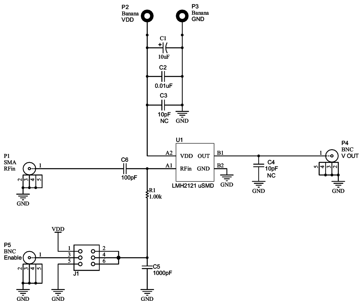
Figure 7. Evaluation Board Schematic
