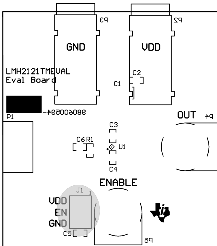
Figure 2. Jumper Positions
