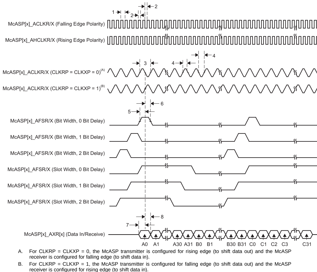
Figure 5-86. McASP Input Timing
