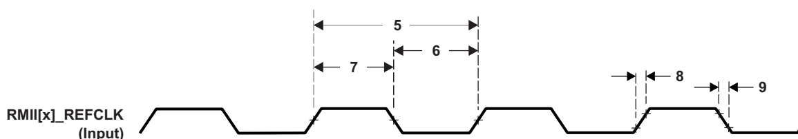
Figure 5-93. MMC[x]_CLK Timing
