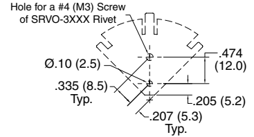
Recommended Mounting Holes
