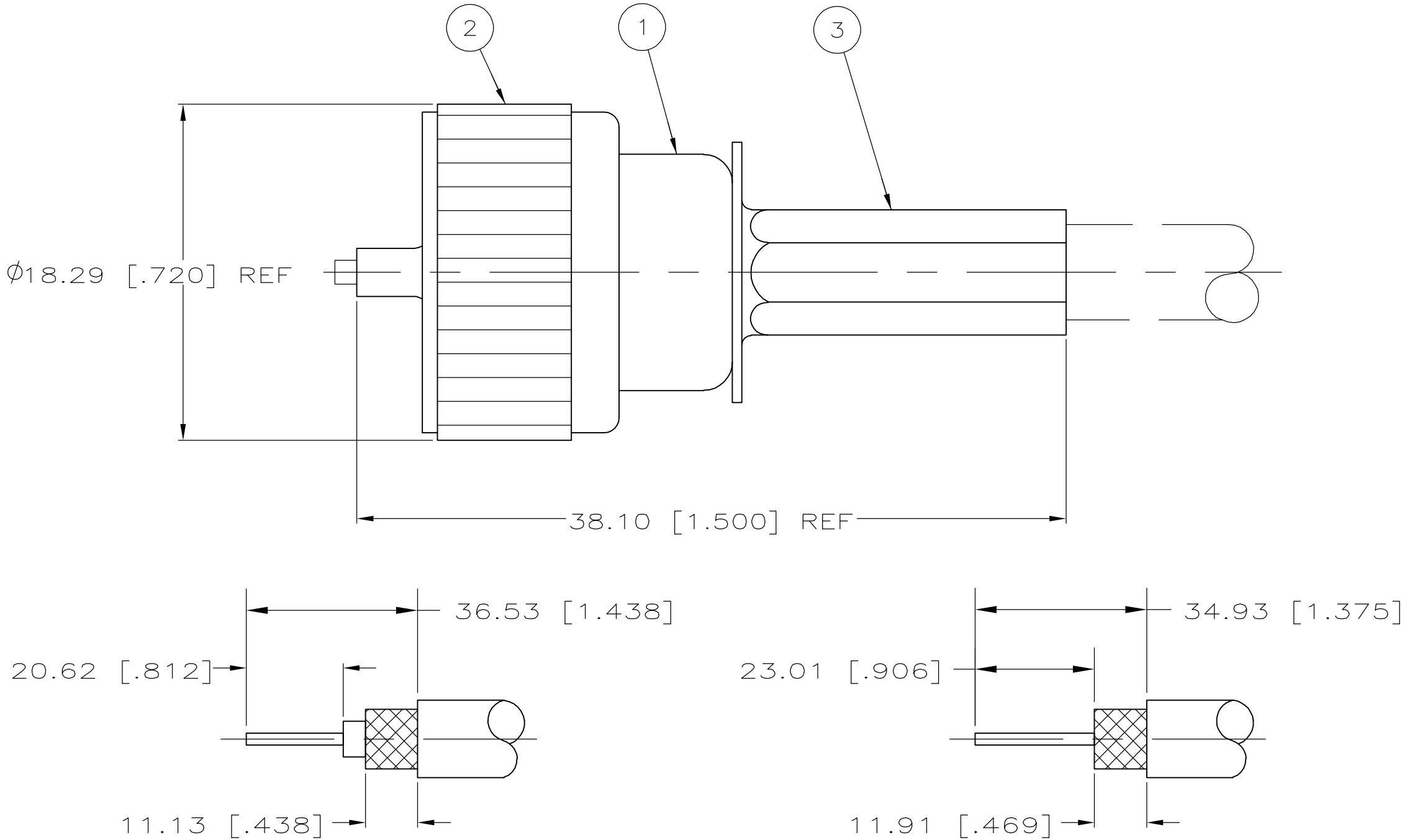
DETAIL A DETAIL B RECOMMENDED STRIP LENGTH
