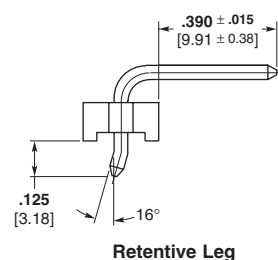
Retentive Leg
