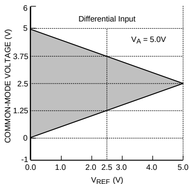
Figure 41. V_{CM} range for Differential Input operation
