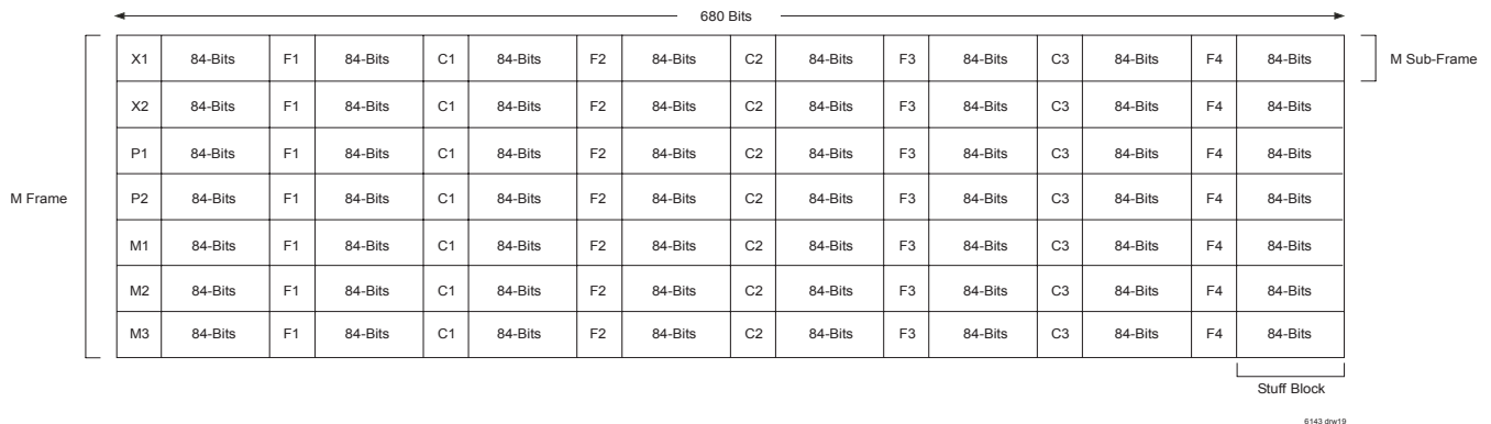
Figure 2 DS3 Frame
