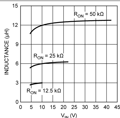
Figure 27. Inductor Selection for V_{OUT} = 0.8\text{ V}
