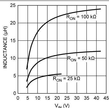
Figure 26. Inductor Selection for V_{OUT} = 3.3\text{ V}
