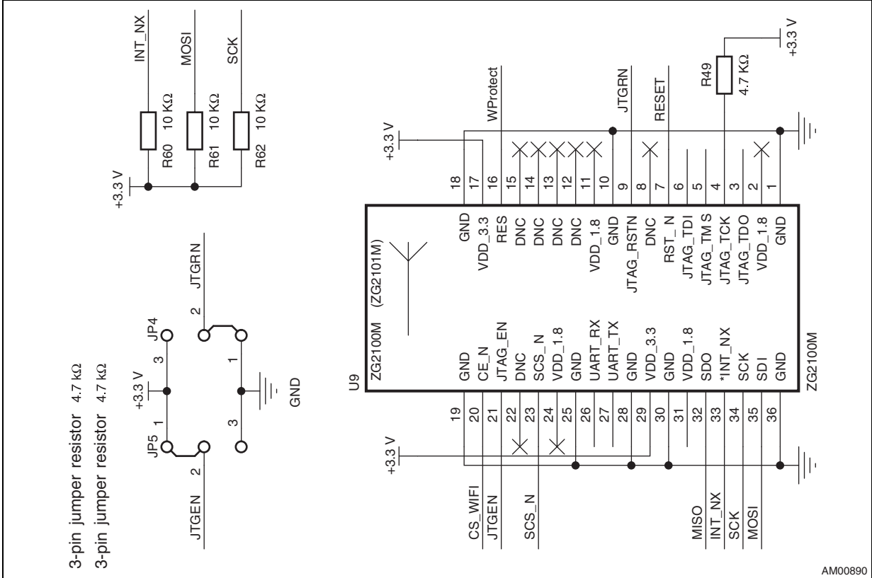
Figure 10. Wi-Fi module-2
