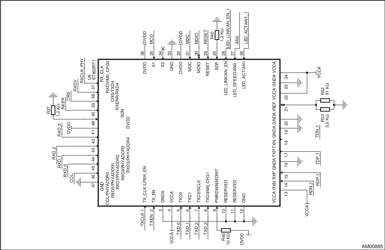
Figure 5. Ethernet - part 1 (PHY pinout)
