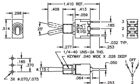
SINGLE POLE
