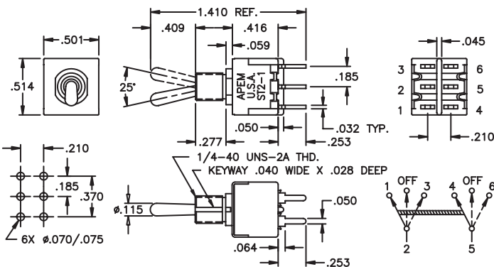
DOUBLE POLE
