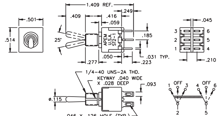
DOUBLE POLE
