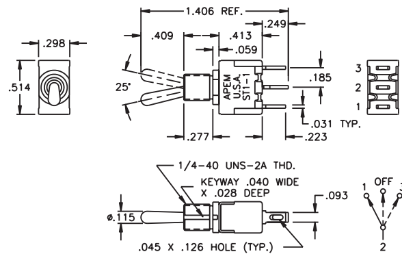
SINGLE POLE
