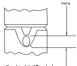
Non-Insulated Terminals
