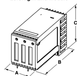
Plug (Daughtercard)
