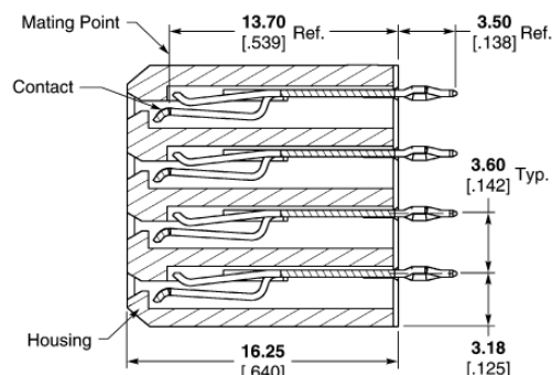
Section Y-Y
