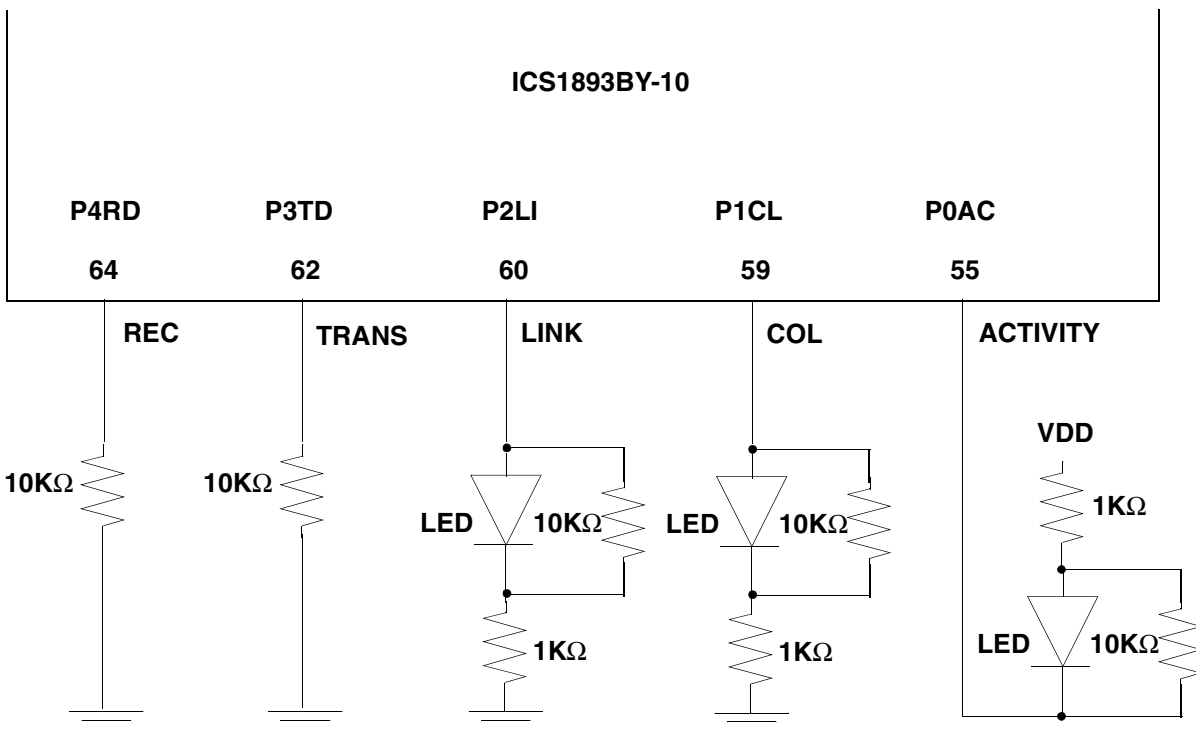
Figure 5-3. ICS1893BY-10 LED - PHY Address
