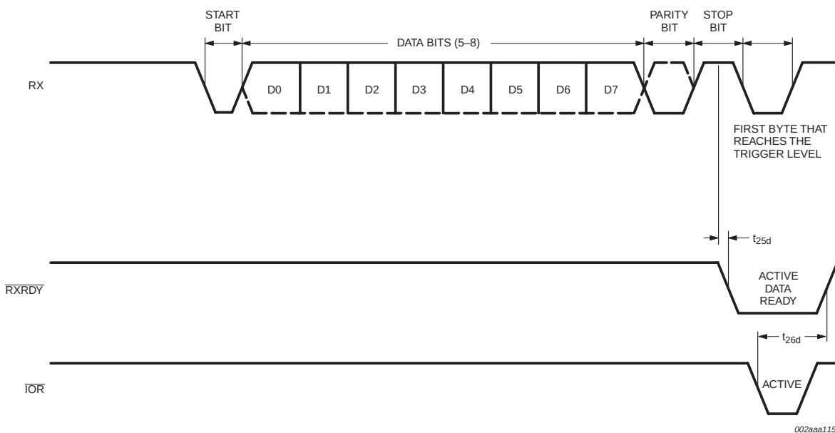
Fig 11. Receive ready timing in FIFO mode.
