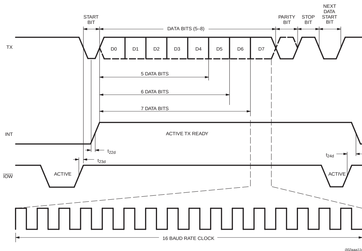
Fig 12. Transmit timing.
