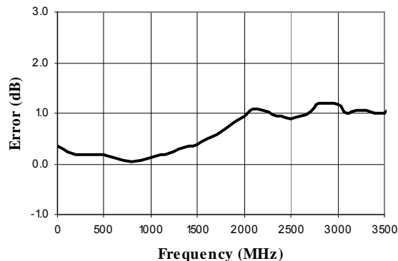
Attenuation Error, Max. Attenuation
