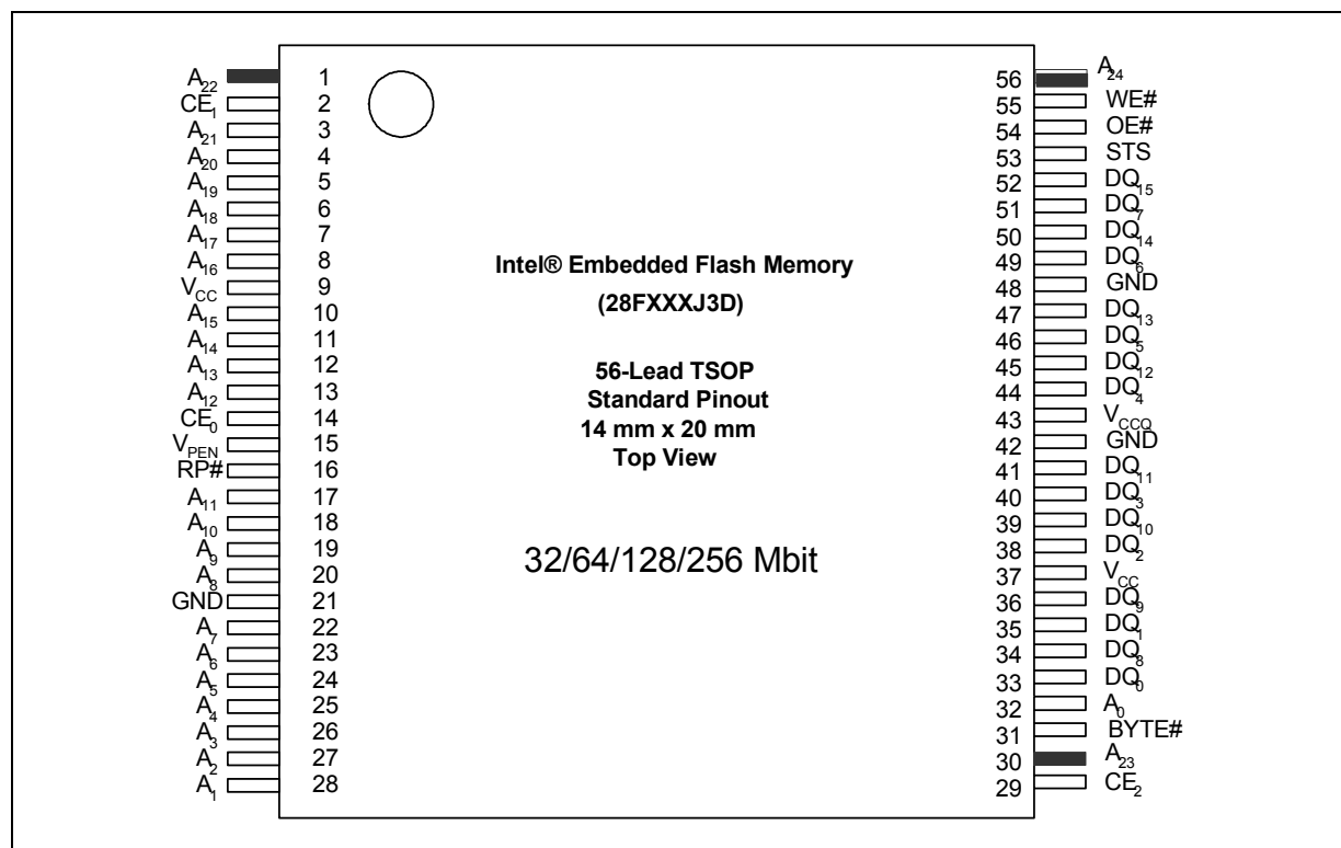
Figure 6: 56-Lead TSOP Package Pinout (32/64/128/256 Mbit)
