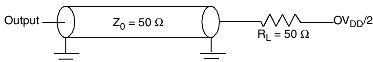
Figure 57. SPI AC Test Load
