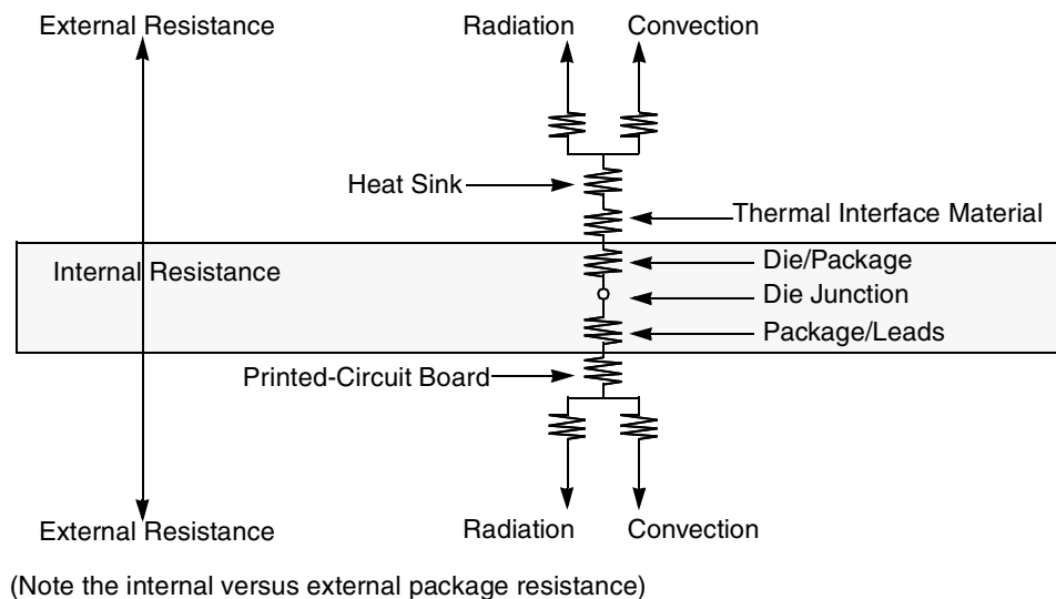
Figure 71. Package with Heat Sink Mounted to a Printed-Circuit Board
