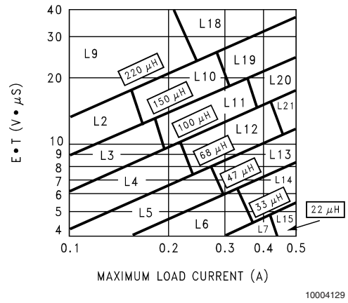
FIGURE 7. LM2674-ADJ
