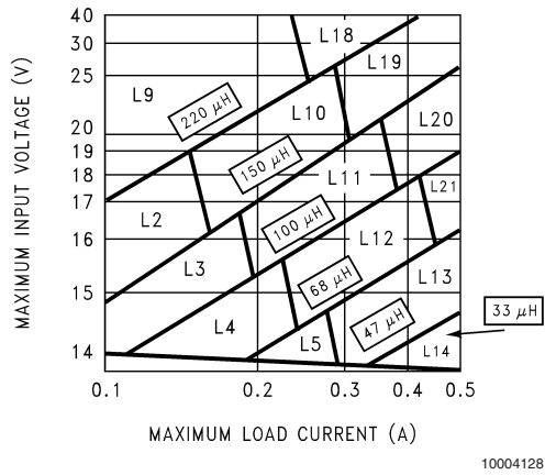
FIGURE 6. LM2674-12
