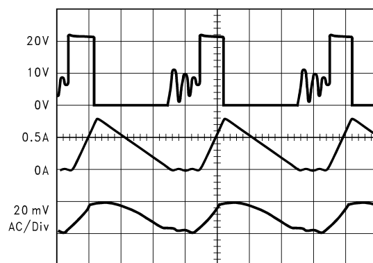
Discontinuous Mode Switching Waveforms V_{IN} = 20V , V_{OUT} = 5V , I_{LOAD} = 300\text{ mA} L = 15\text{ }\mu\text{H} , C_{OUT} = 68\text{ }\mu\text{F} (2x), C_{OUT}ESR = 25\text{ m}\Omega
