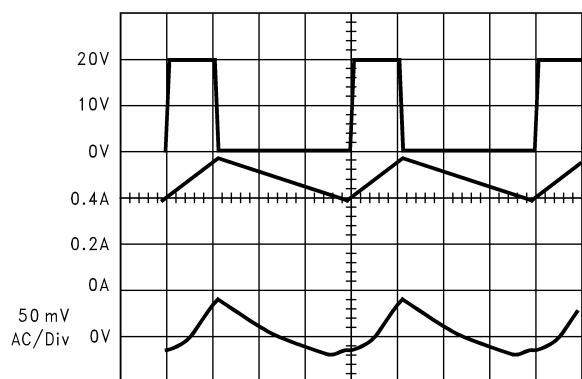
Continuous Mode Switching Waveforms V_{IN} = 20V , V_{OUT} = 5V , I_{LOAD} = 500\text{ mA} L = 100\text{ }\mu\text{H} , C_{OUT} = 100\text{ }\mu\text{F} , C_{OUT}ESR = 0.1\Omega
