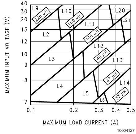
FIGURE 5. LM2674-5.0
