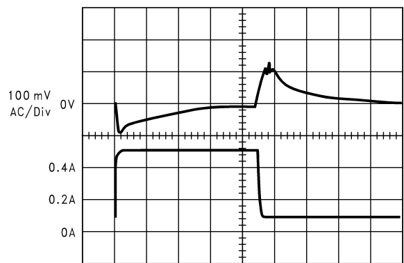
Load Transient Response for Continuous Mode V_{IN} = 20V , V_{OUT} = 5V , L = 100\text{ }\mu\text{H} , C_{OUT} = 100\text{ }\mu\text{F} , C_{OUT}ESR = 0.1\Omega
