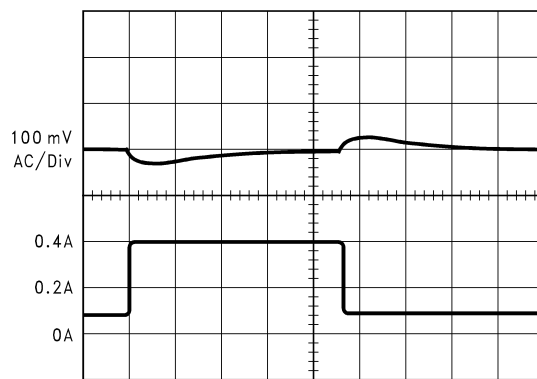
Load Transient Response for Discontinuous Mode V_{IN} = 20V , V_{OUT} = 5V , L = 47\text{ }\mu\text{H} , C_{OUT} = 68\text{ }\mu\text{F} , C_{OUT}ESR = 50\text{ m}\Omega
