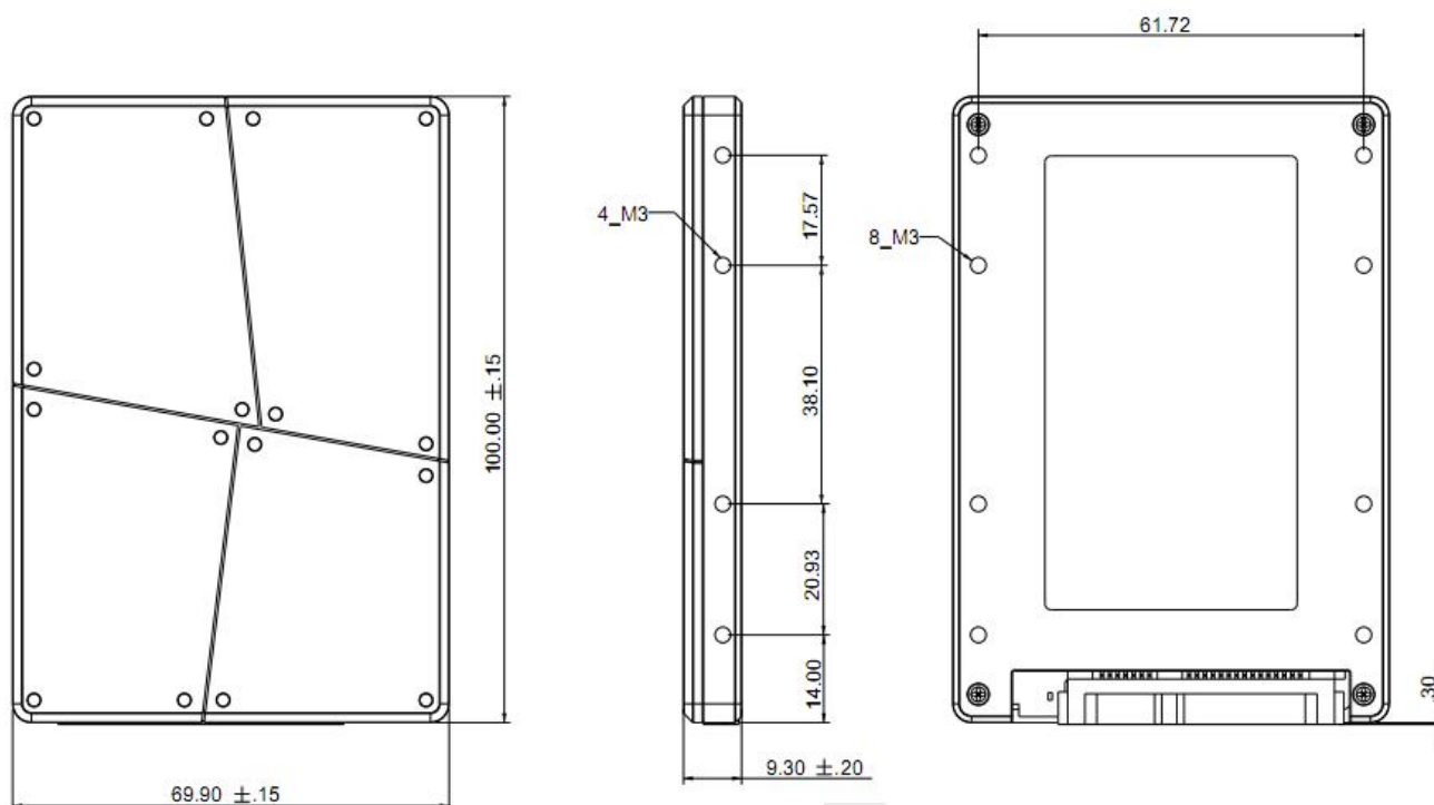
Figure 6-1 SAFD 25P-M w/Metal Housing physical dimensions
