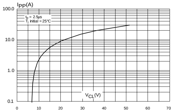
Figure 6: Clamping voltage versus peak pulse current (typical values, rectangular waveform)
