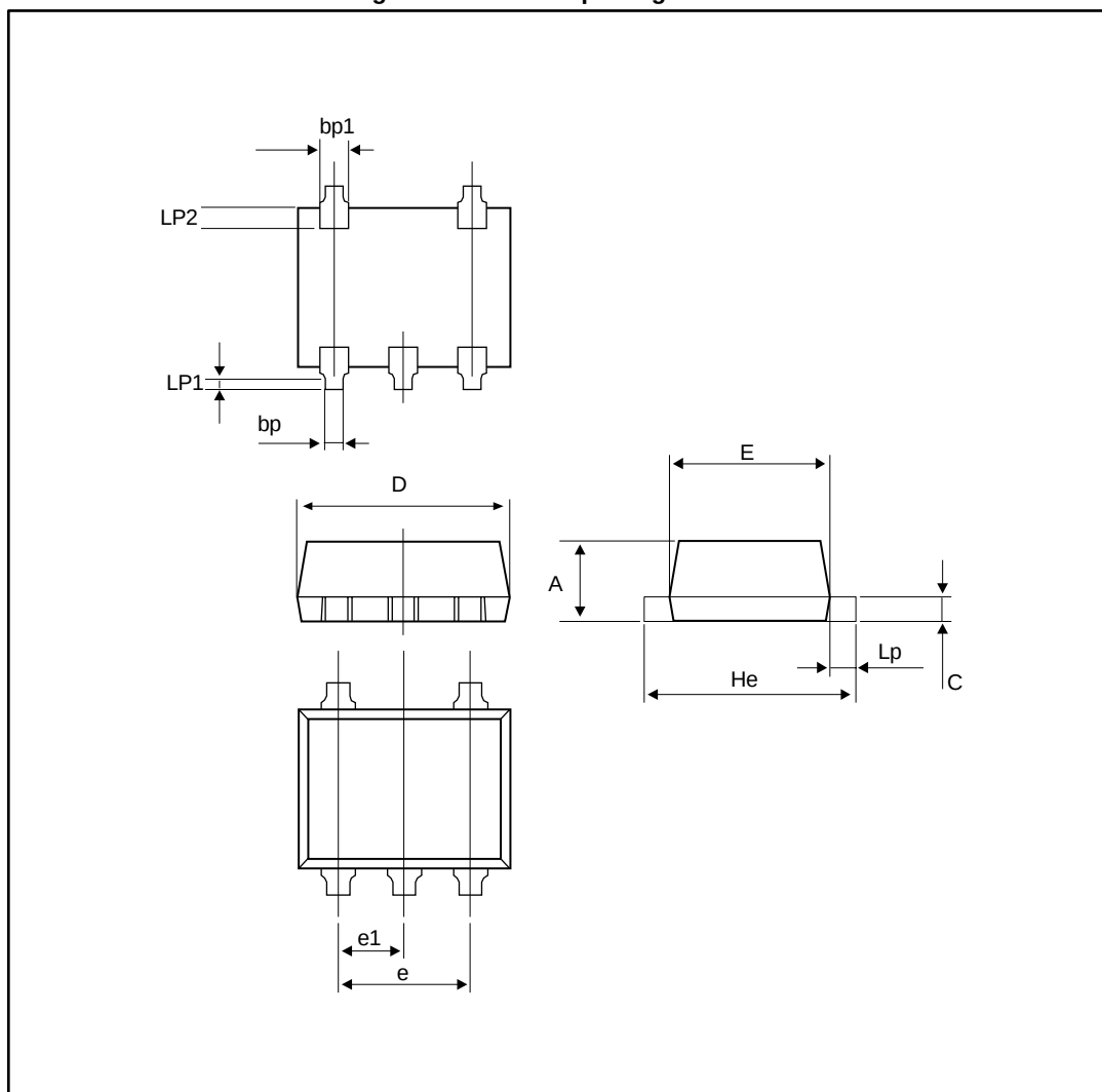
Figure 13: SOT-665 package outline
