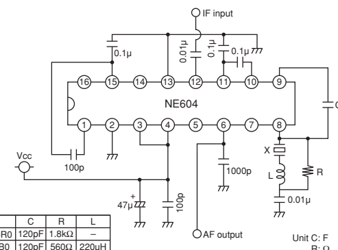
NE604N
